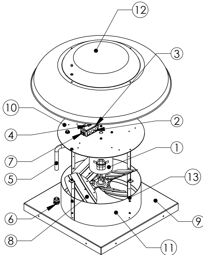
Direct Drive - Down Blast Axial Fan - Motor Information.
